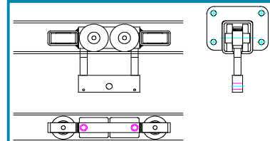
reinforced trolley
